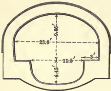
FIG. 5. OLD STYLE.
